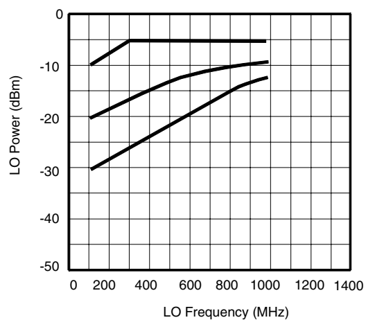
Figure 7-15. Typical useful LO Power Range versus LO Frequency at T_{amb} = 25^{\circ}\text{C}
